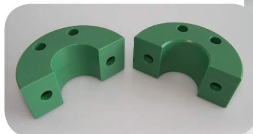
Split bearing block machined from Sustamid® 6G OL
