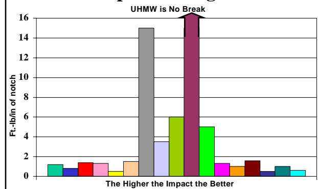
Impact Strength
